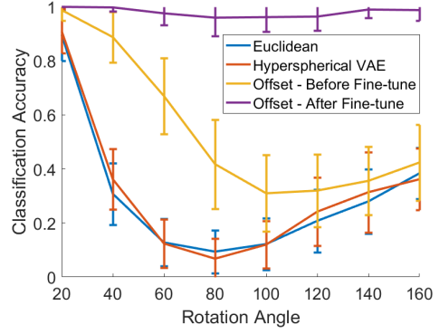
Figure 5: Nearest neighbor classification accuracy of rotated test digits.
